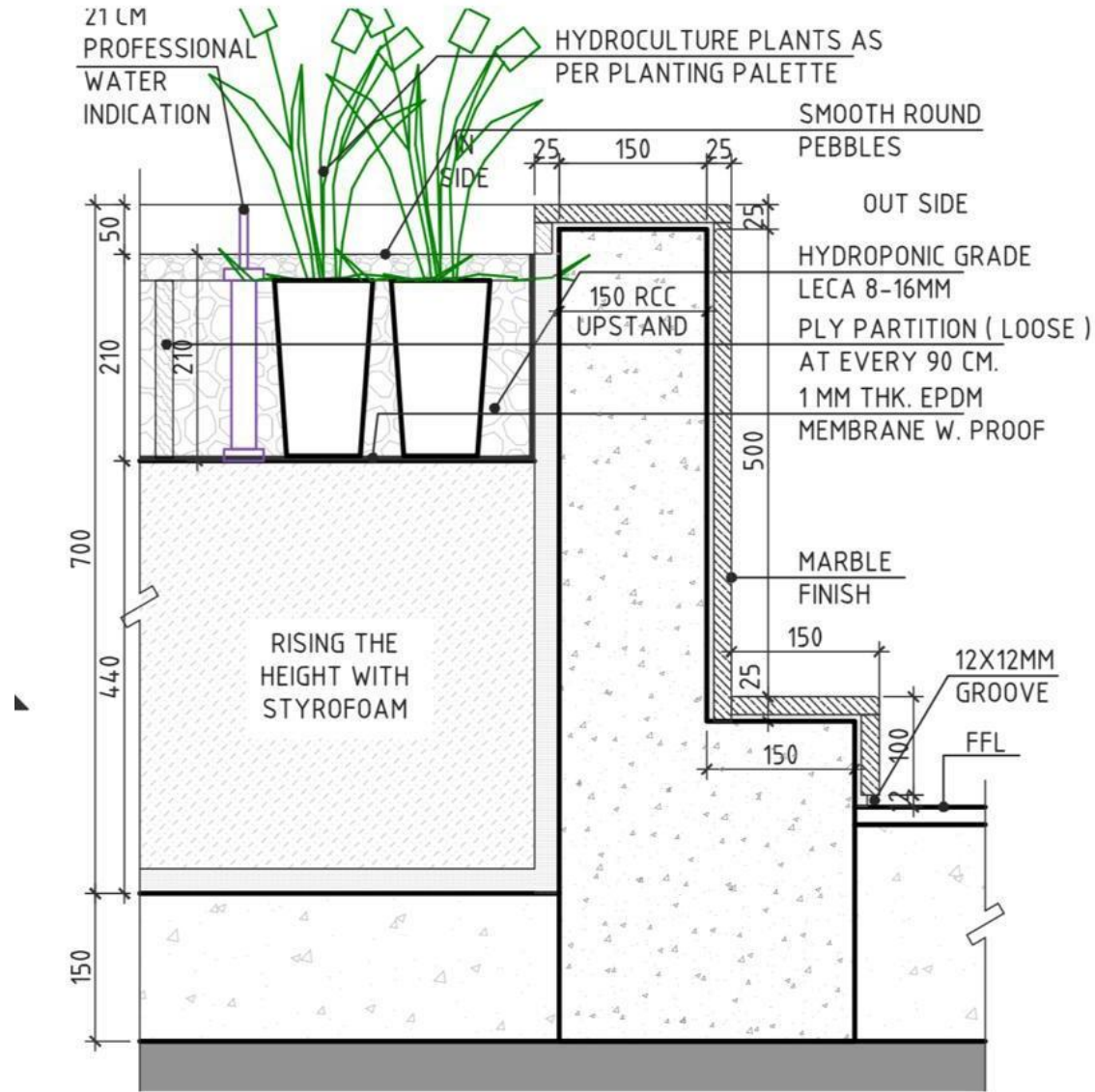
TYPICAL DETAIL B SCALE 1:10
